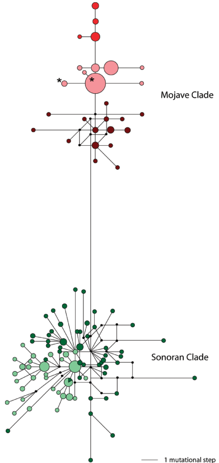
FIG. 4. —Median-joining network of mtDNA control region sequences for Chaetodipus penicillatus . Sonoran clade indicated in green with light green indicating northern distribution and dark green indicating southern distribution. Mojave clade indicated in red shades with identified subgroups (burgundy = Southern Mojave subgroup, red = Western Mojave subgroup, pink = Northern Mojave subgroup). The length of connection lines between haplotypes is proportional to number of mutational changes, with the shortest connection line representing 1 mutational change. Black dots indicate median vectors inferred from the data. Circle size reflects number of individuals exhibiting a given haplotype progressing from smallest ( n = 1 ) to largest ( n = 8 ). The asterisks represent haplotypes found in individuals from Death Valley.
