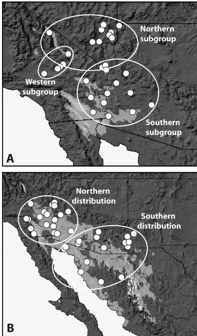
FIG. 6.—Enlarged views of ecological niche models of latest glacial maximum climatic condition for A) Mojave clade and B) Sonoran clade with overlays of sample localities where each clade was identified. The 3 subclades of the Mojave clade (A) and the 2 regional distributions of haplotypes from the Sonoran clade (B) are indicated (note that 1 haplotype was shared between the 2 regions).
